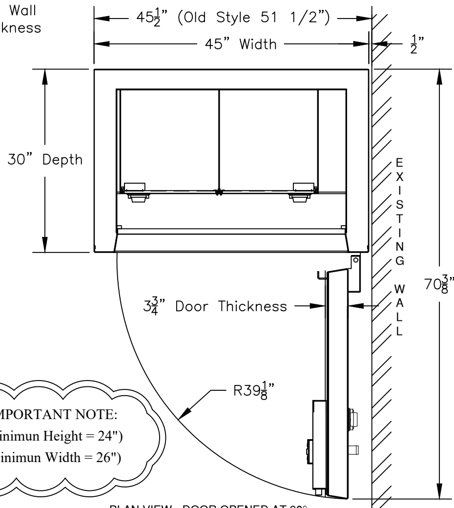
PLAN VIEW - DOOR OPENED AT 90°
