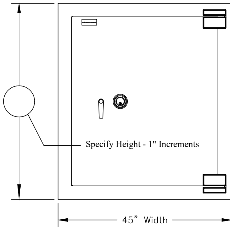
FRONT ELEVATION
